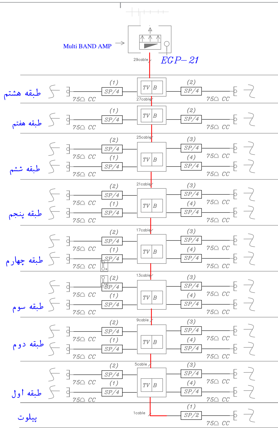
CENTRAL ANTENNA RISER DIAGRAM
